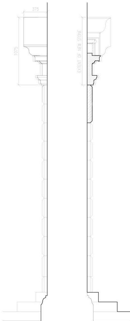
Section and Elevation of new garden door entrance.
