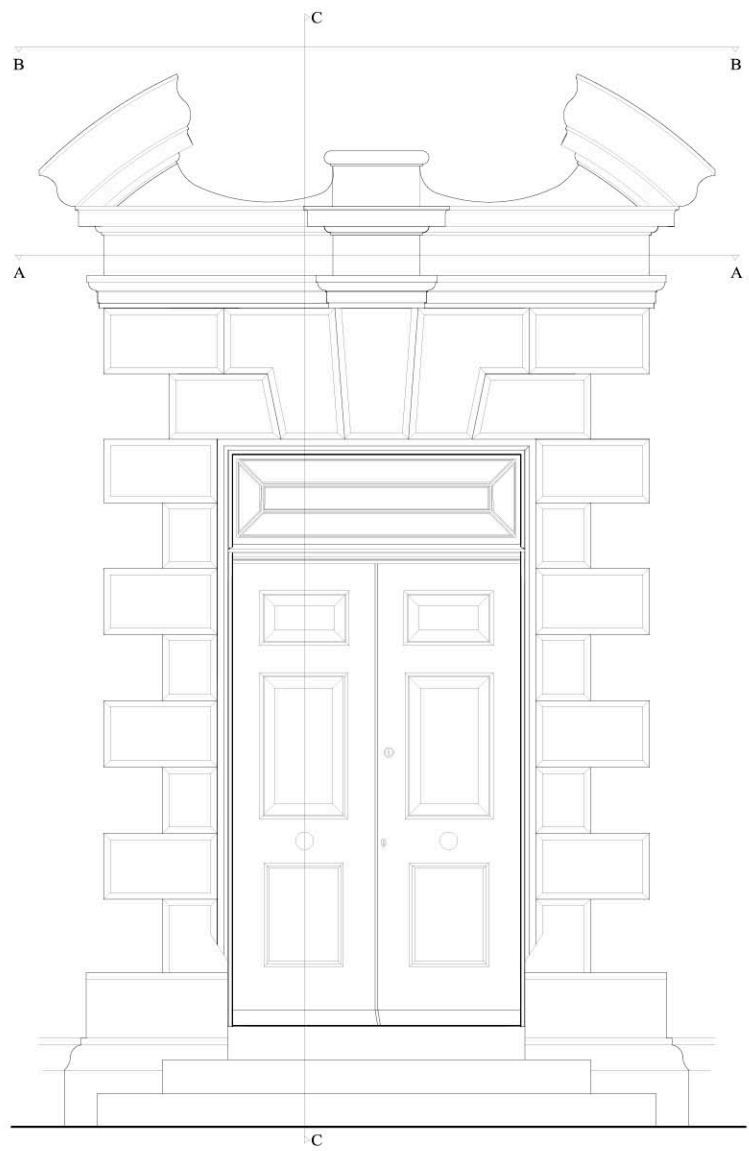
Elevation of new garden entrance, showing new stone pediment details.
