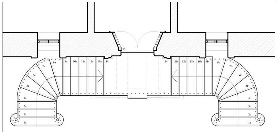
Detail plan of forestairs.
