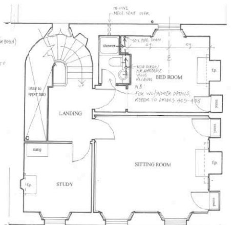
Proposed lower & upper flat plan.
