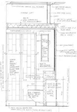
Section of en-suite bathroom.
