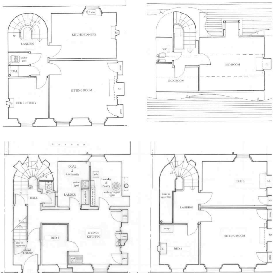
Existing lower & upper flat plan.
